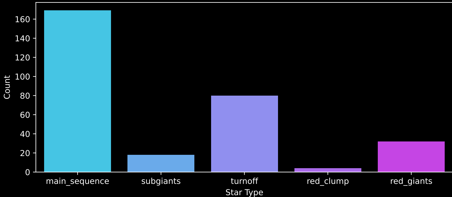
GALAH DR4 Field: [70] Count plot of Star Type
