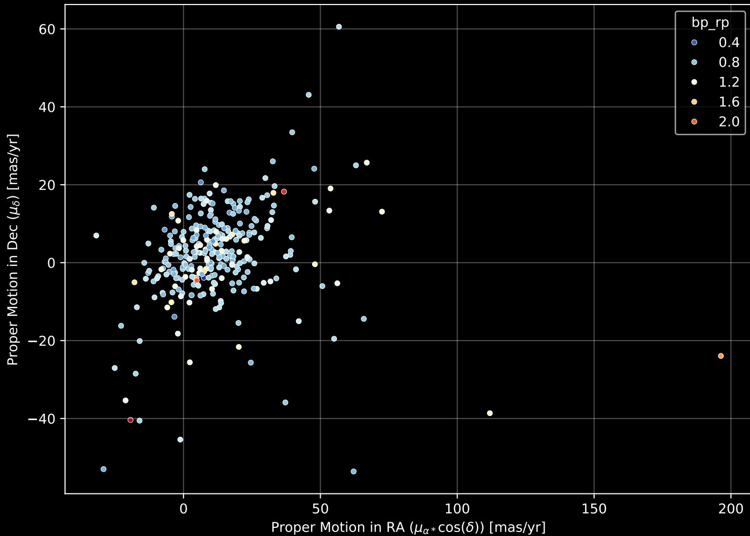
GALAH DR4 Field: [70] Proper Motion Diagram (n= 303)
