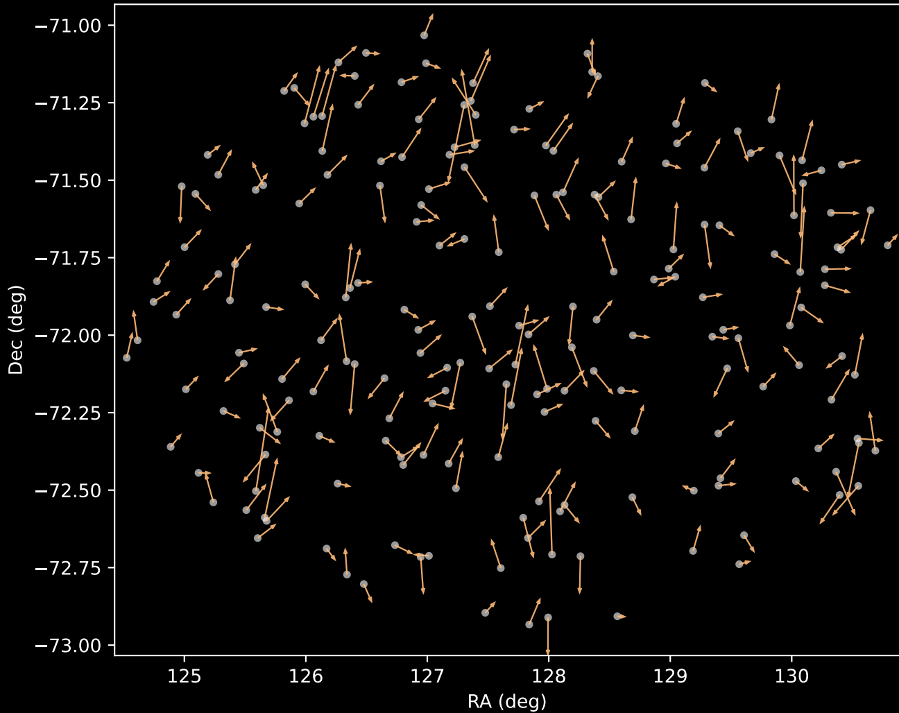
GALAH DR4 Cluster 3 Proper Motion Vectors (n=202)
