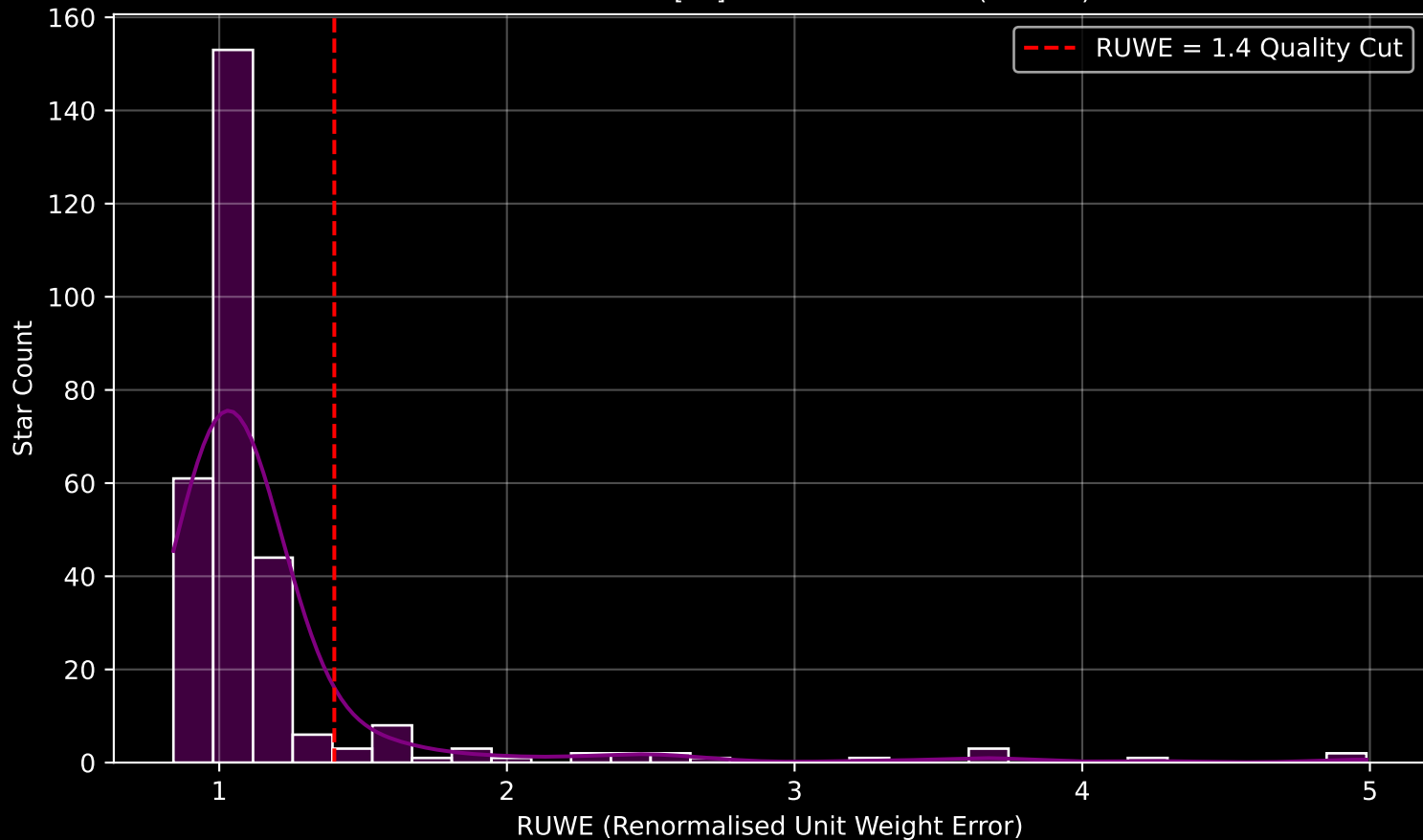
GALAH DR4 Field [70] RUWE Distribution (n= 294)
