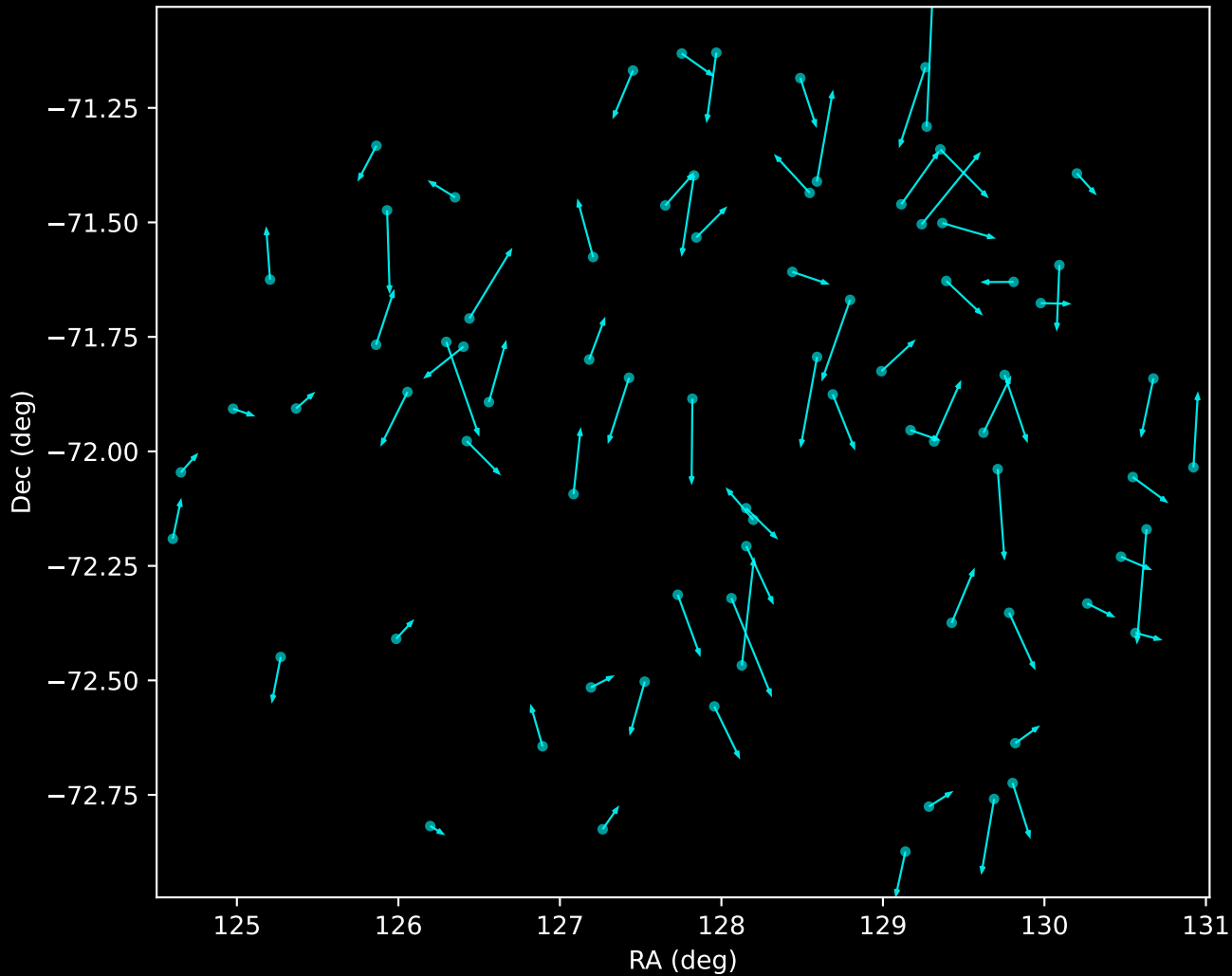
GALAH DR4 Noise Stream Proper Motion Vectors (n=78)
