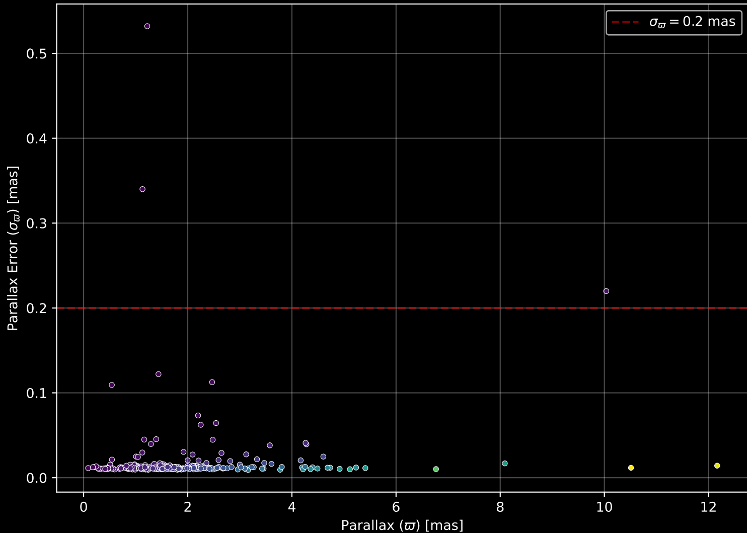
GALAH DR4 Field: [70] Parallax Quality (n= 303)
